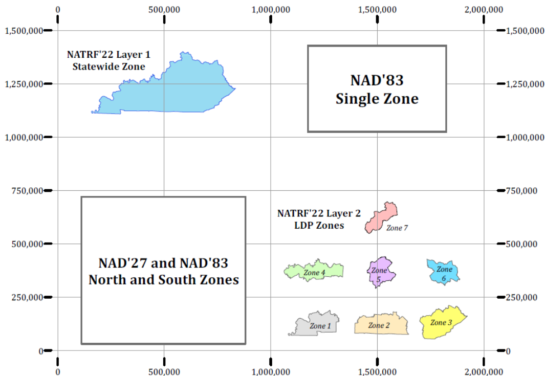
Figure 1.7.2.6 Coordinate space comparison for all KSPCS 2022 zones, with those defined on pre-2022 datums represented by their respective extents and in aggregate where they overlap.
