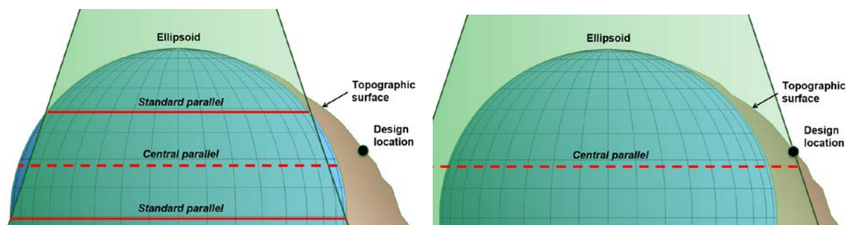
Figure 2.3.1 Typical SPCS situation (for LCC projection) on left. Projection is secant to ellipsoid, with developable surface below topographic surface. Figure on the right depicts a situation in which SPCS is scaled “to ground” at design location. Central parallel in same location as original SPCS; note developable surface inclined with respect to topographic surface. (Dennis, 2019).
