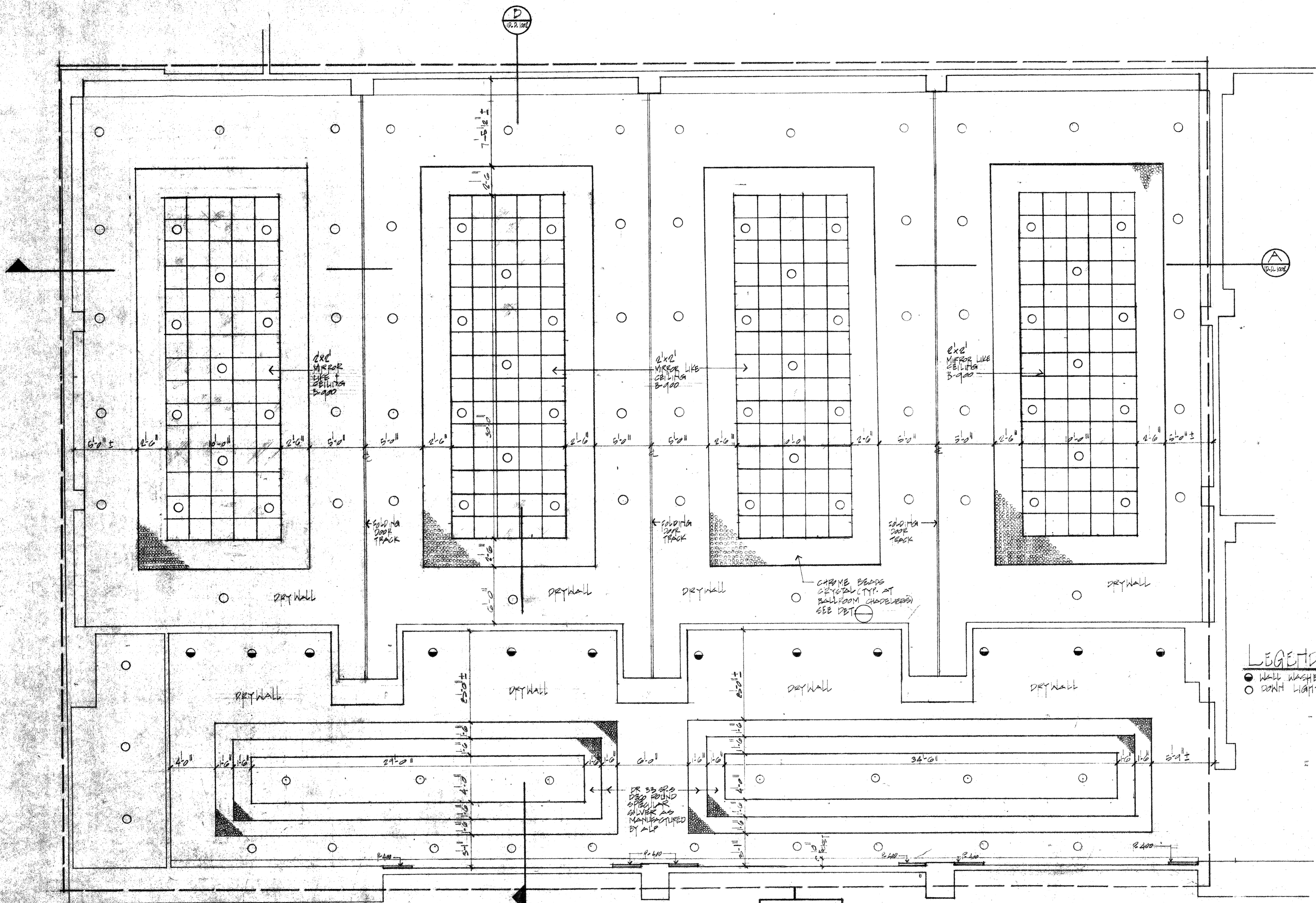
REFLECTED CEILING PLAN SCALE: 1/4" = 1'-0"
