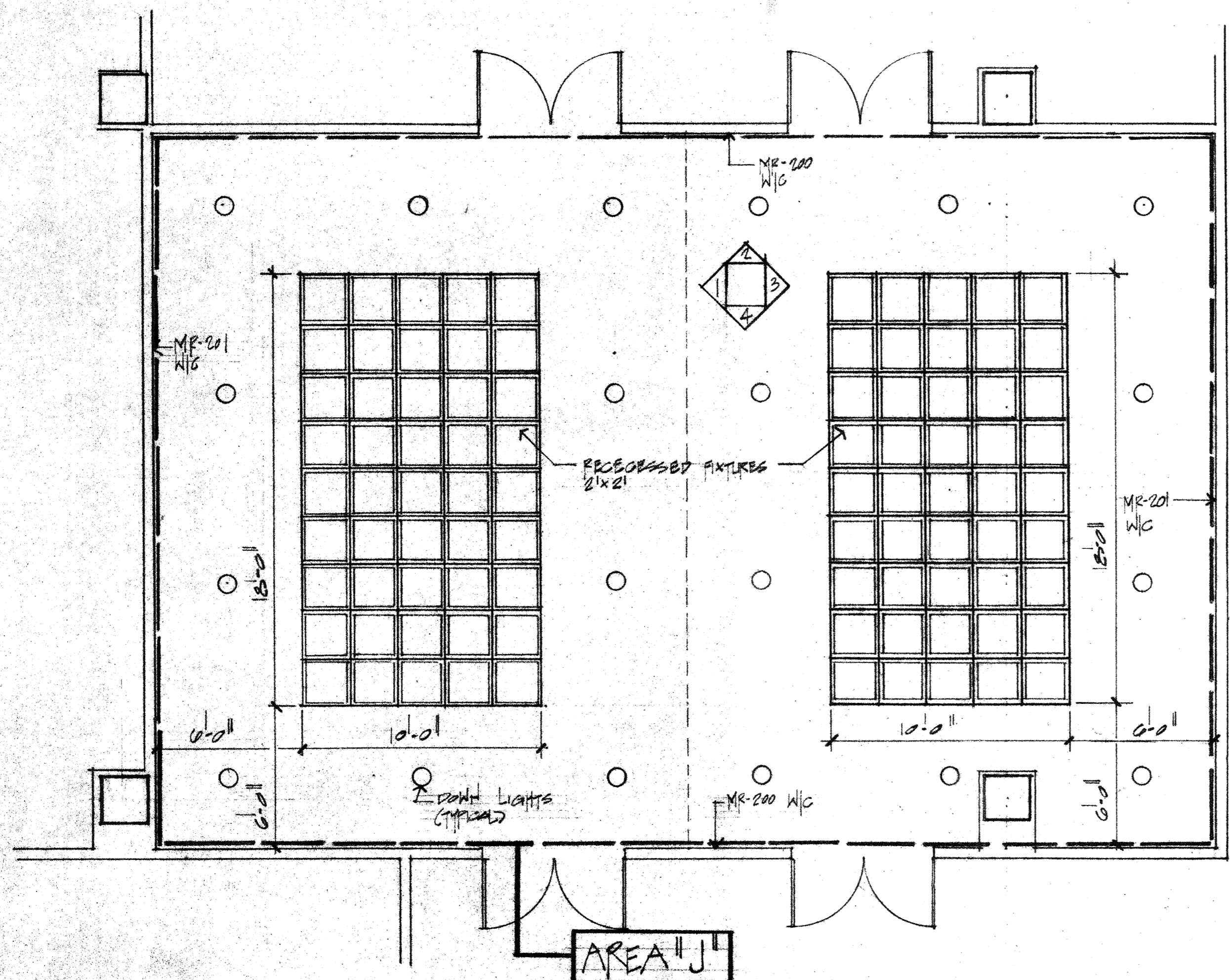
MEETING ROOMS 'A' & 'D' REFLECTED CEILING SCALE: 1/4" = 1'-0"
