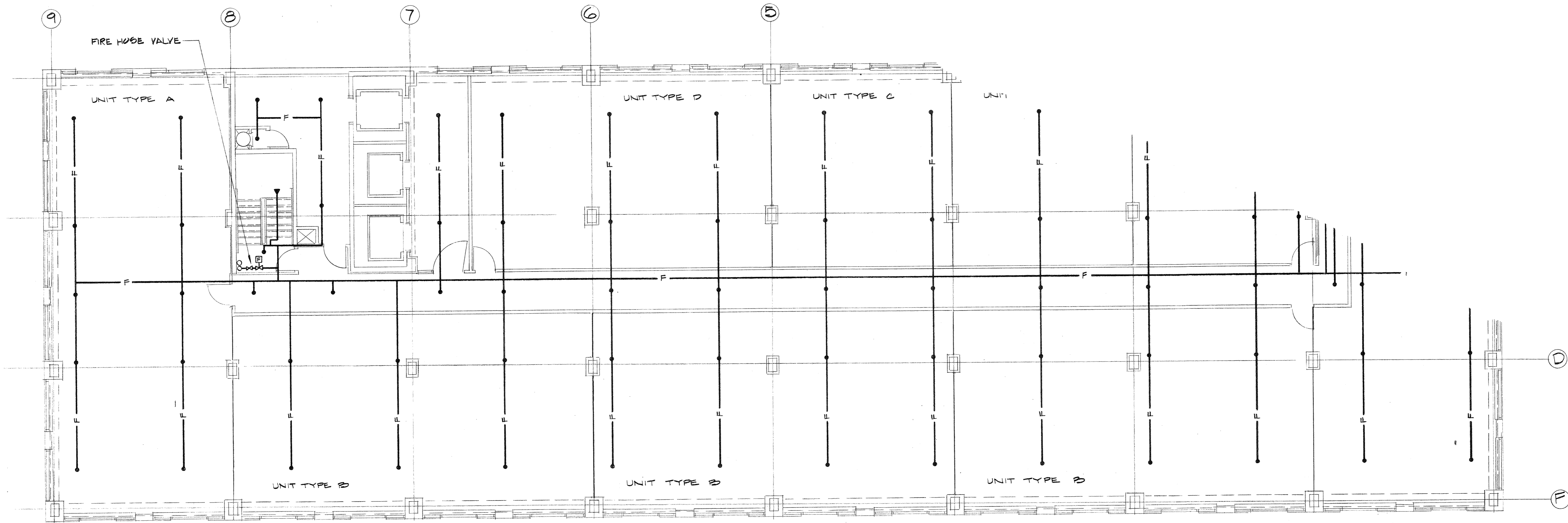
SPRINKLER PLAN - 9 TH FLOOR - CONDOMINIUMS SCALE: 1/8" = 1'-0"
