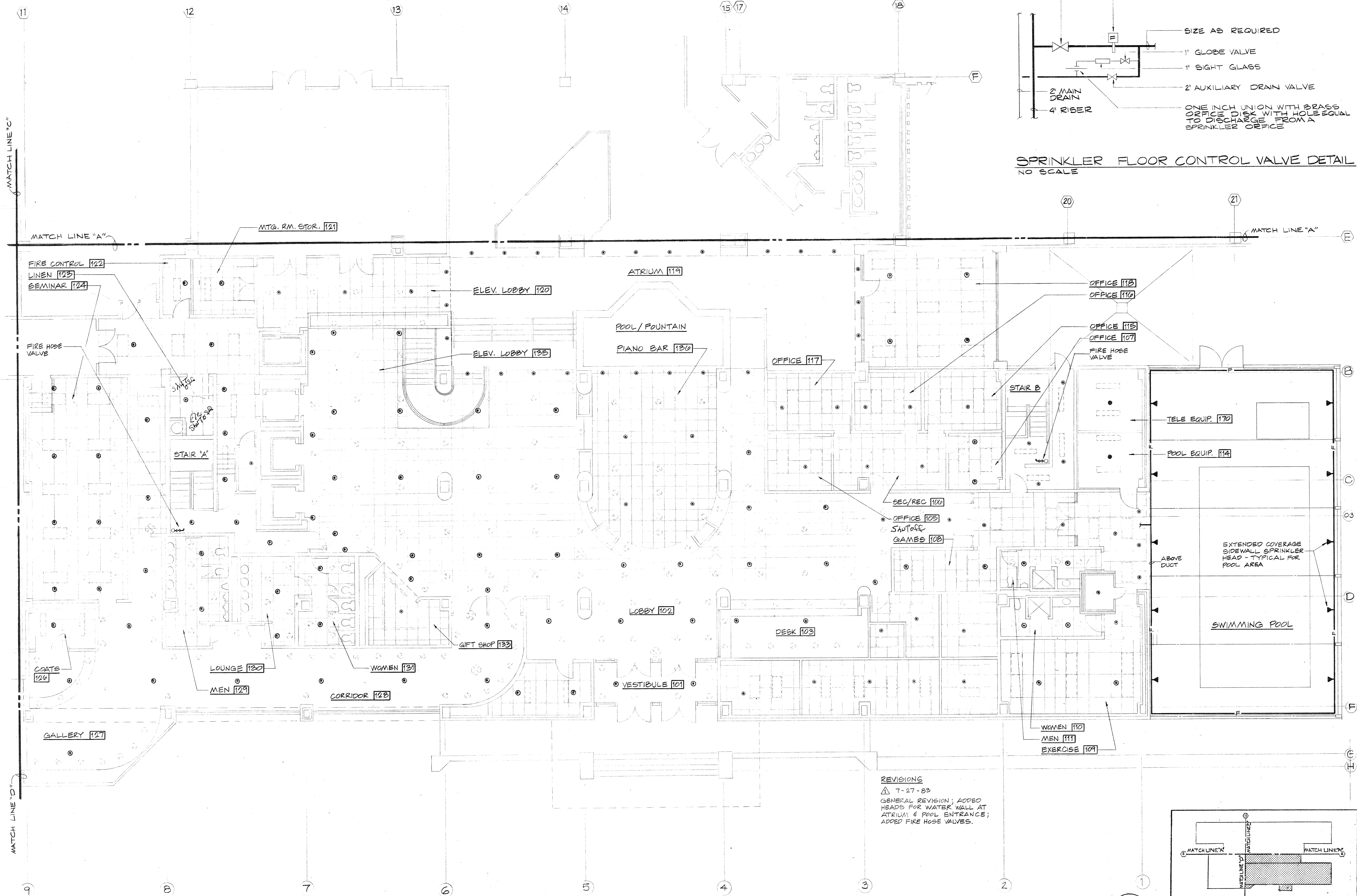
PARTIAL SPRINKLER PLAN - LOBBY / MEZZANINE LEVEL SCALE: 1/8" = 1'-0"
