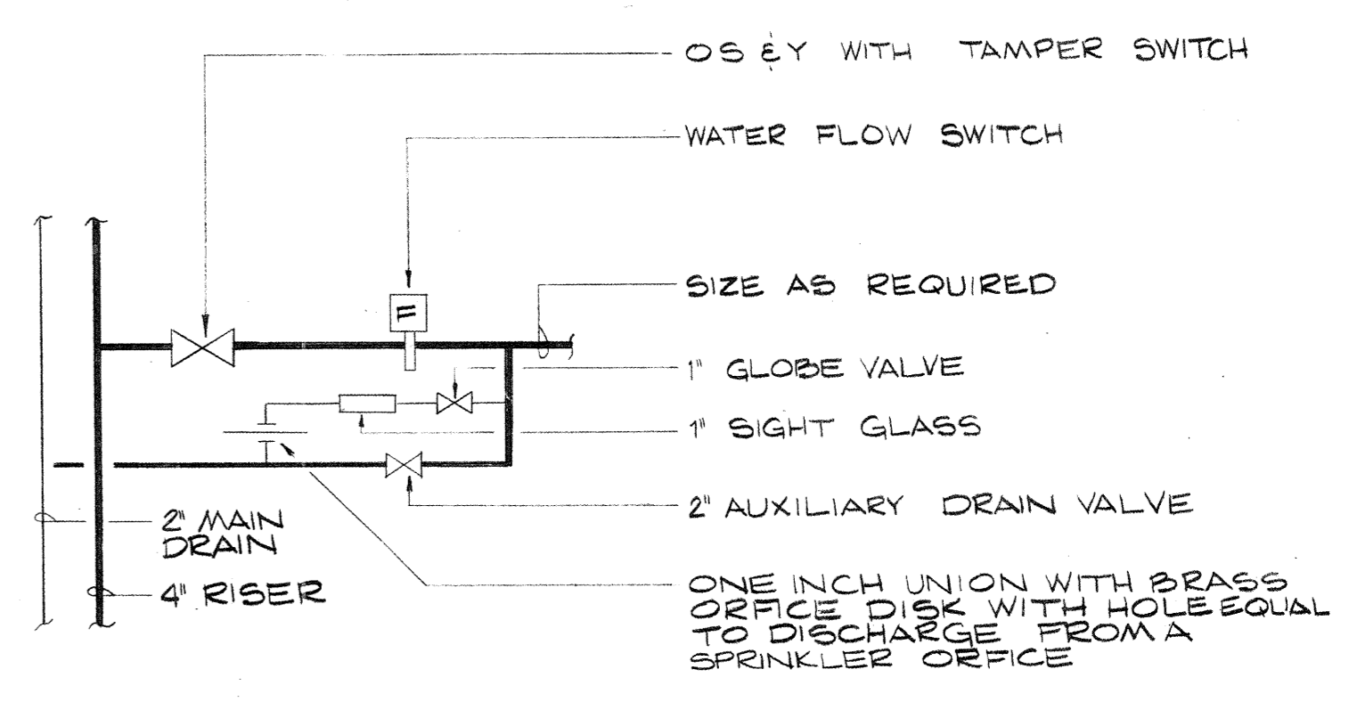
SPRINKLER FLOOR CONTROL VALVE DETAIL NO SCALE
