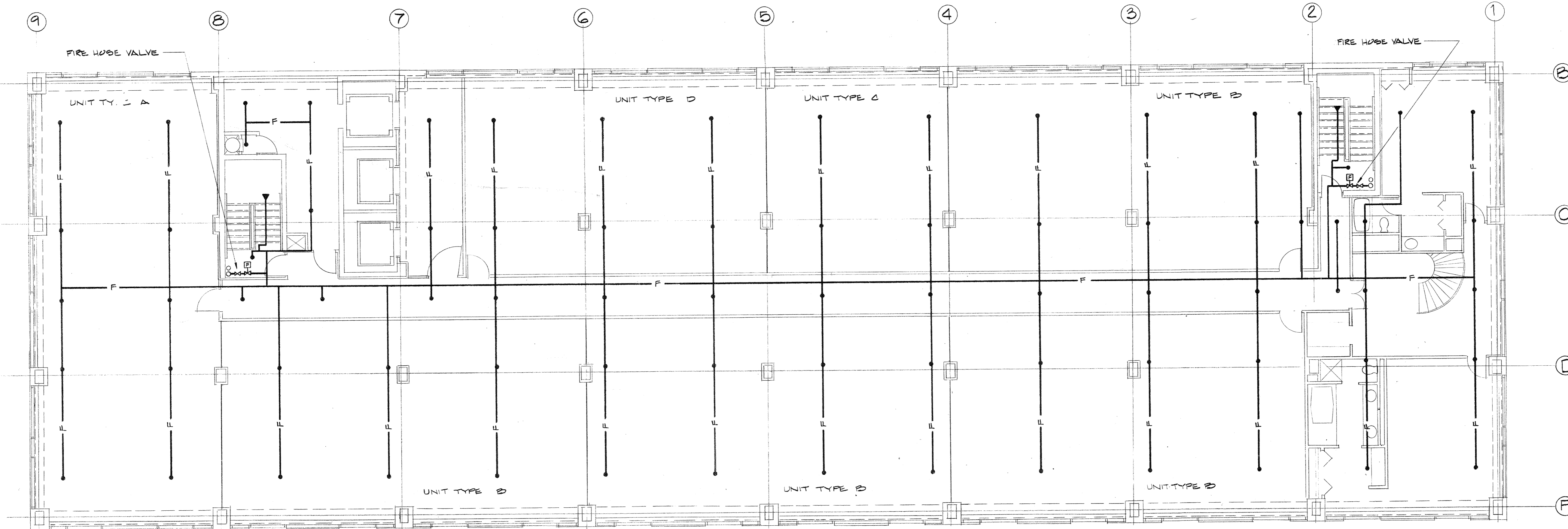
SPRINKLER PLAN - 10 TH FLOOR - CONDOMINIUMS SCALE: 1/8" = 1'-0"
