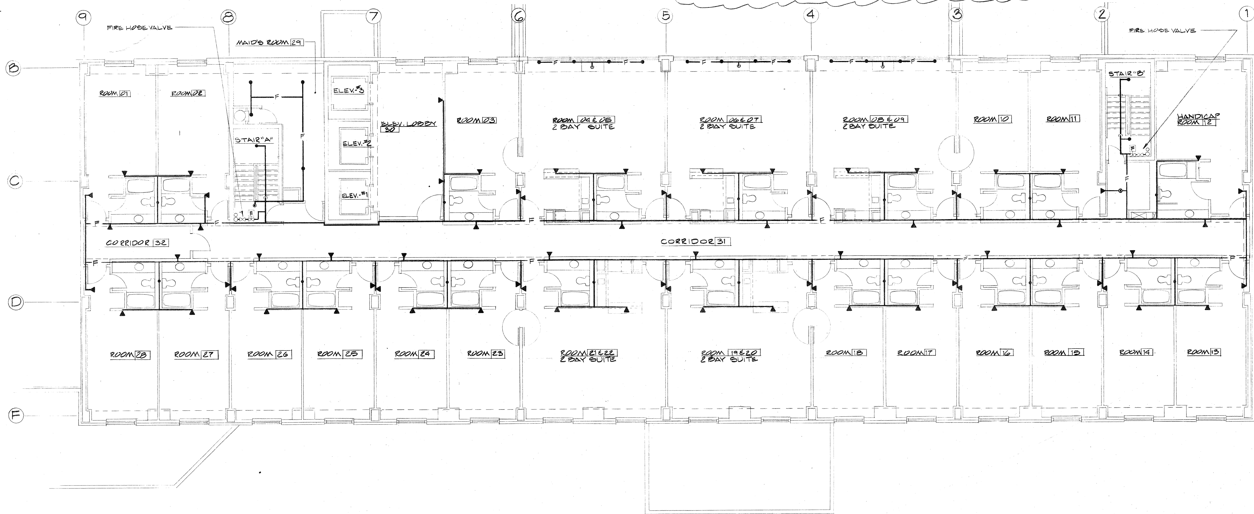
SPRINKLER PLAN - MECHANICAL ROOM SCALE: 1/8" = 1'-0"
